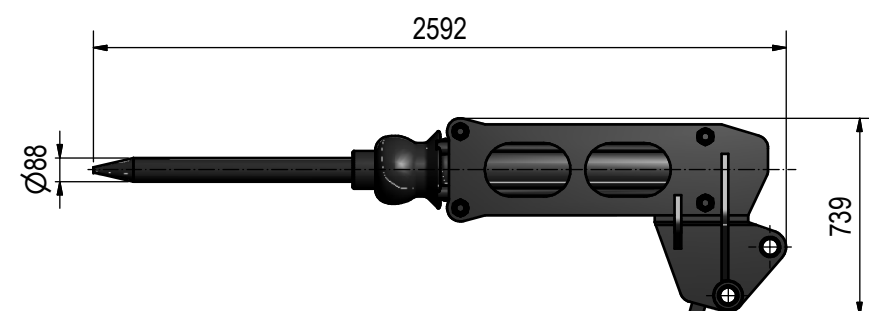
PNEUNMATIC HAMMER (1:20)
